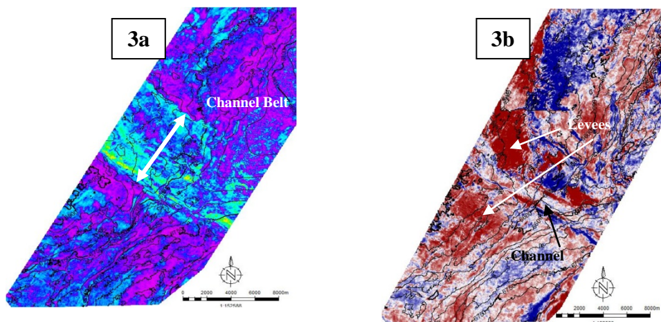
Figure 3: a) RMS amplitude at Paleocene Top (window: +20ms to -20ms). 3b) Amplitude extracted in a 10ms window, 40ms below Paleocene Top.
