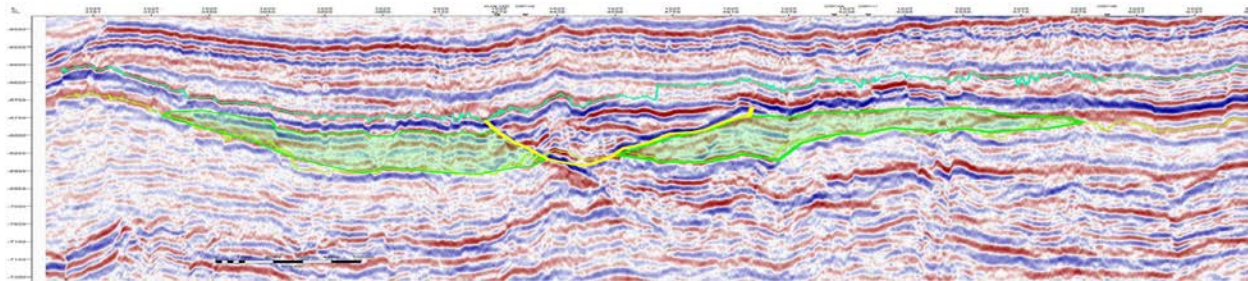
Figure 2: NW-SE line, 3D Area A, showing Paleocene multistoried channel with well-developed levees. Positive compactional relief within channel, indicating presence of coarser clastics.
